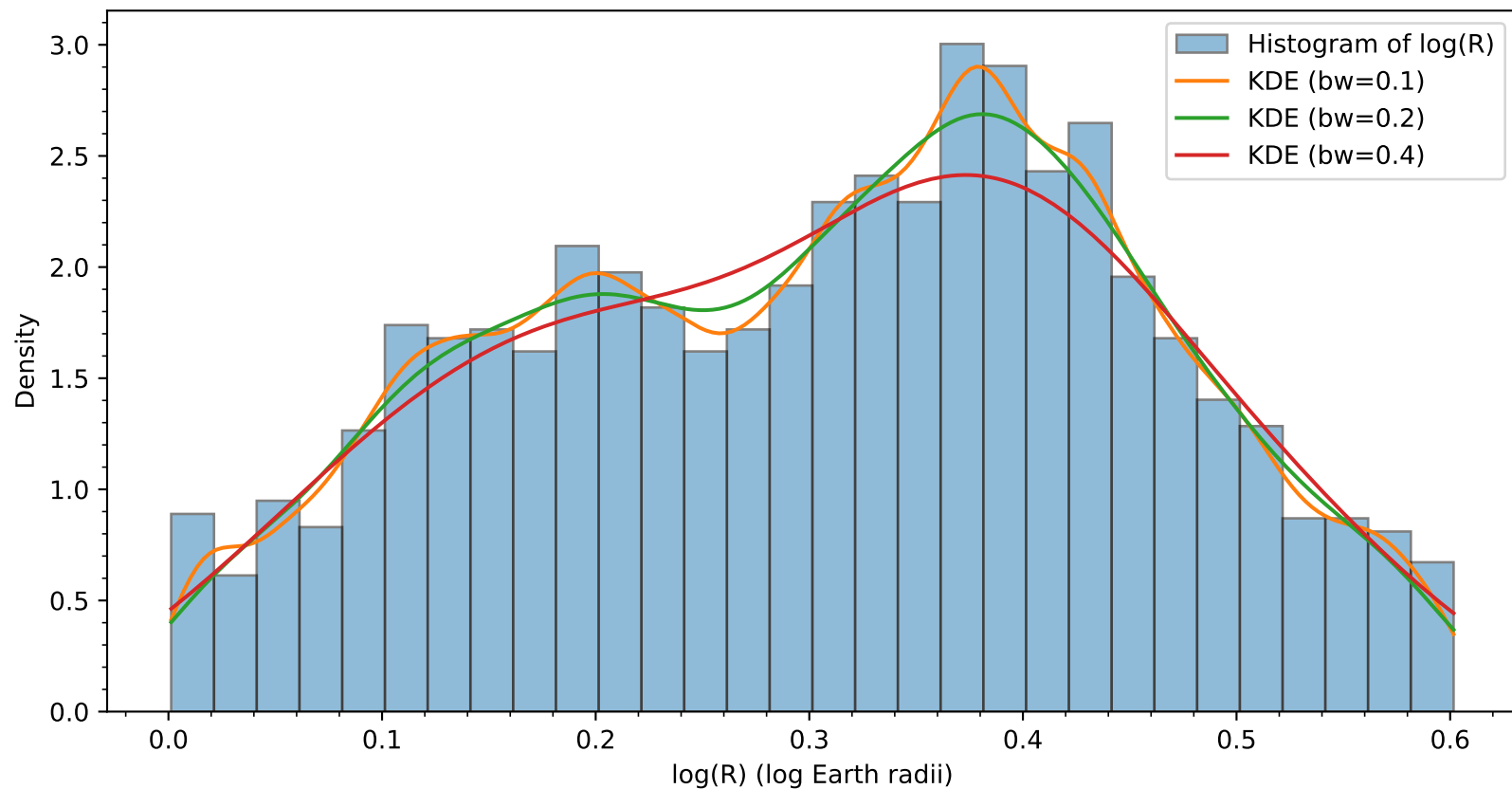
Distribution of Planet Radii
